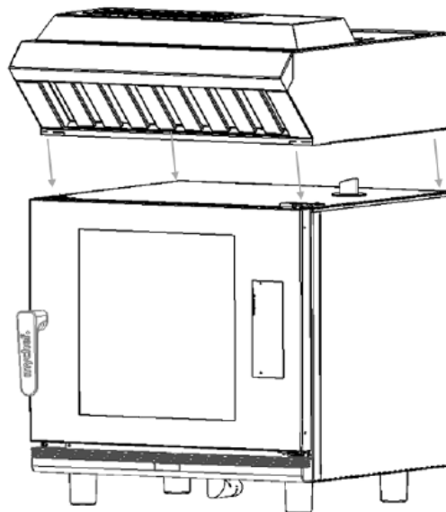
Figure 3. Positioning of the condensation hood
